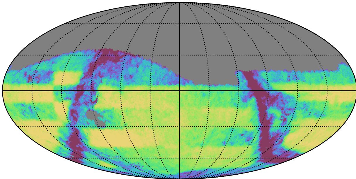
too_5_4v3.4_10yrs Yr 3-4 i band: Exgal_CoaddM5
