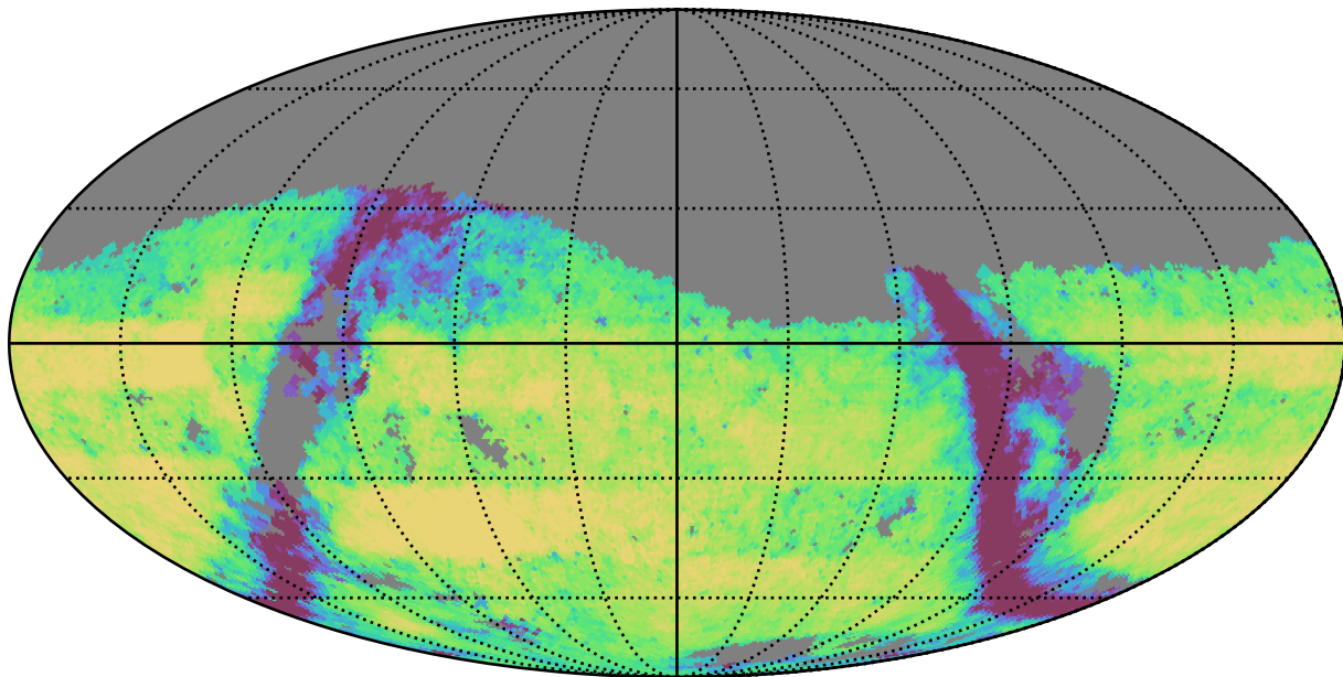
too_5_4v3.4_10yrs Yr 3-4 g band: Exgal_CoaddM5
