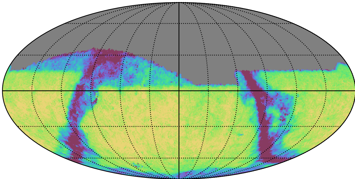
too_5_4v3.4_10yrs Yr 1 z band: Exgal_CoaddM5
