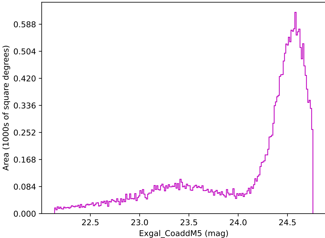
too_5_4v3.4_10yrs Yr 1 z band: Exgal_CoaddM5
