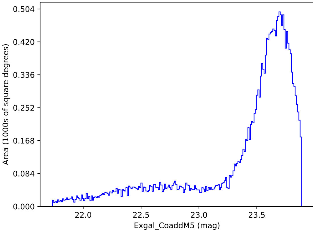
too_5_4v3.4_10yrs Yr 1 y band: Exgal_CoaddM5
