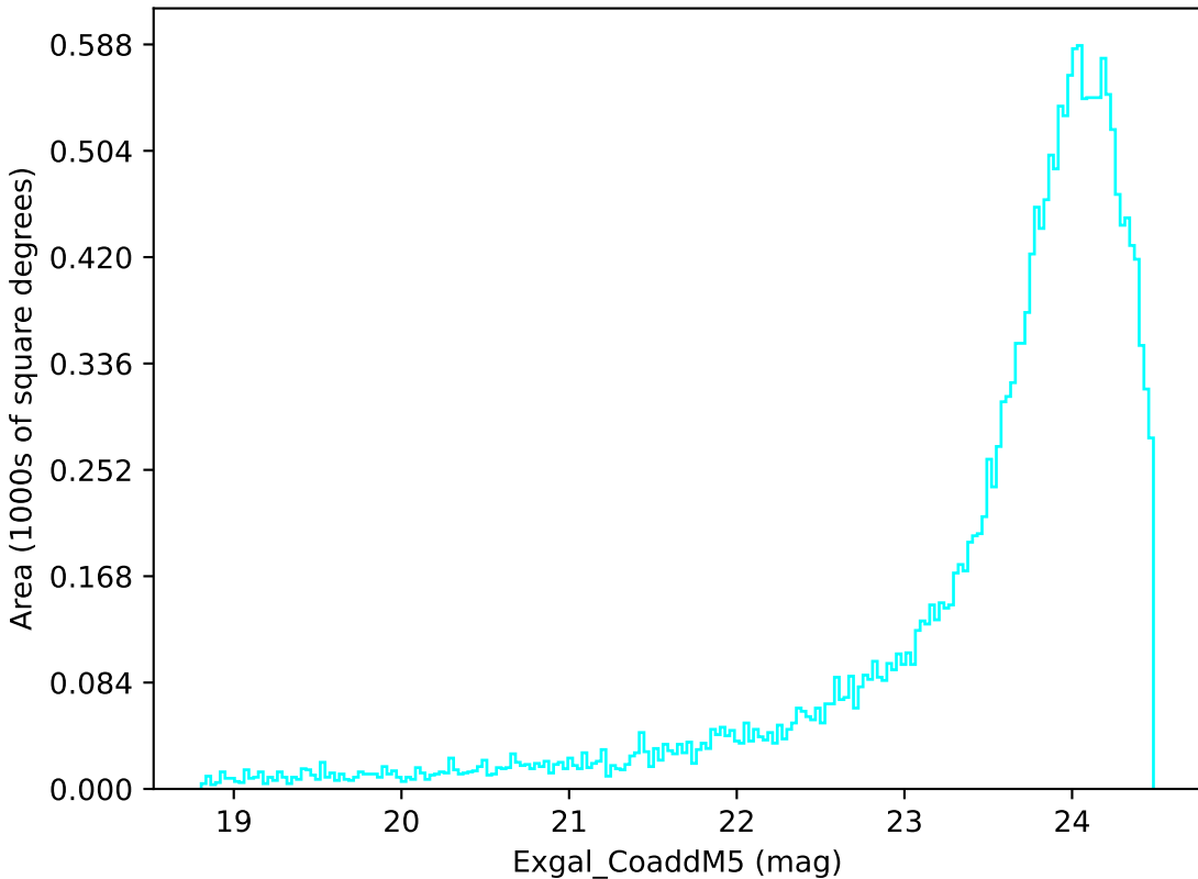
too_5_4v3.4_10yrs Yr 1 u band: Exgal_CoaddM5
