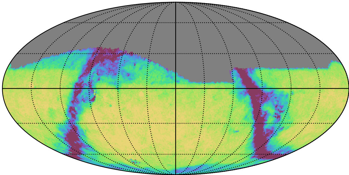
too_5_4v3.4_10yrs Yr 1 r band: Exgal_CoaddM5
