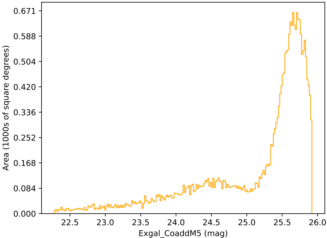
too_5_4v3.4_10yrs Yr 1 r band: Exgal_CoaddM5
