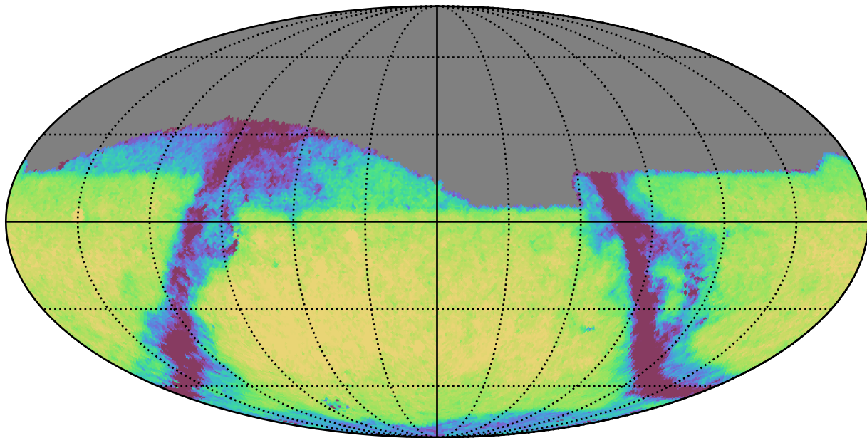
too_5_4v3.4_10yrs Yr 1 i band: Exgal_CoaddM5
