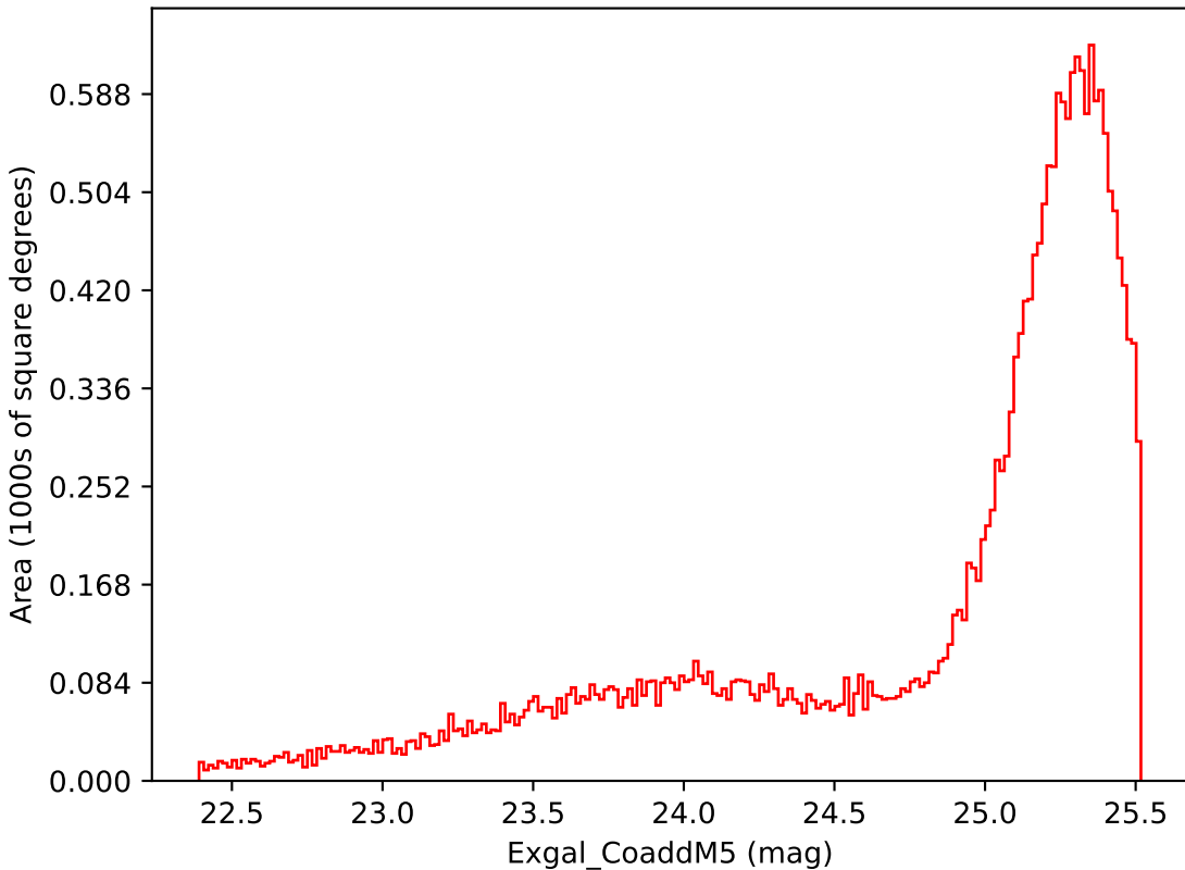
too_5_4v3.4_10yrs Yr 1 i band: Exgal_CoaddM5
