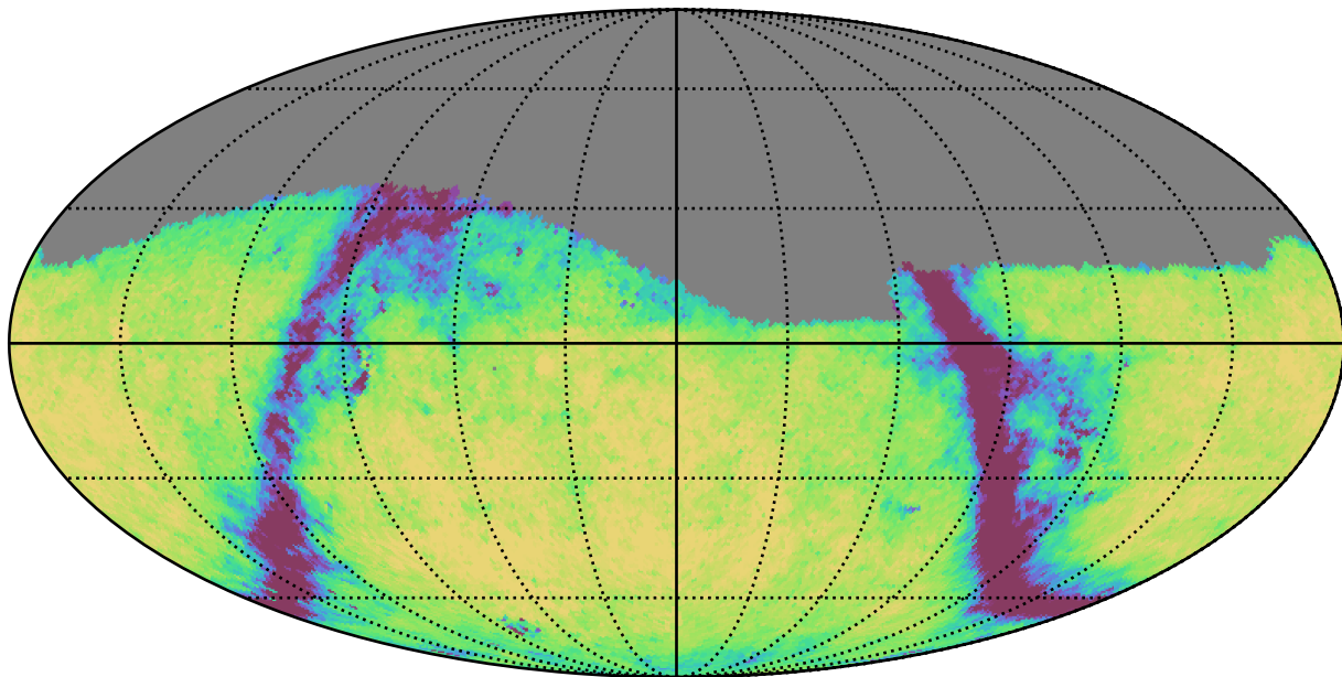
too_5_4v3.4_10yrs Yr 1 g band: Exgal_CoaddM5
