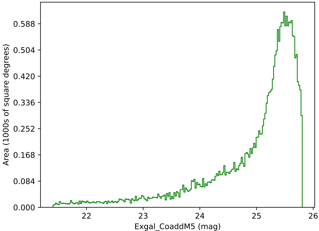
too_5_4v3.4_10yrs Yr 1 g band: Exgal_CoaddM5
