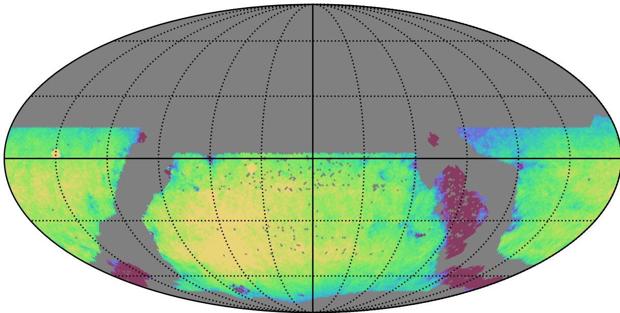
too_5_4v3.4_10yrs WFD z band: Exgal_CoaddM5
