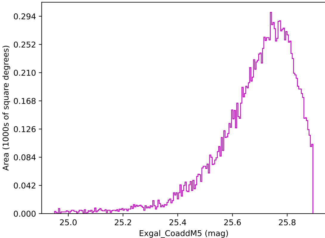
too_5_4v3.4_10yrs WFD z band: Exgal_CoaddM5
