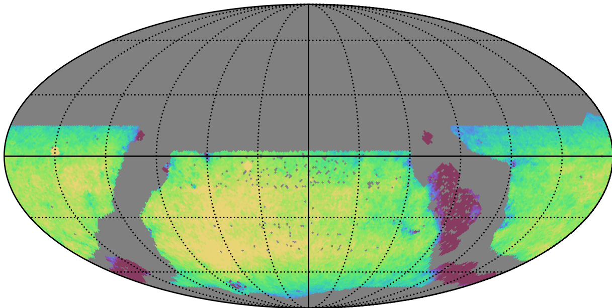
too_5_4v3.4_10yrs WFD y band: Exgal_CoaddM5
