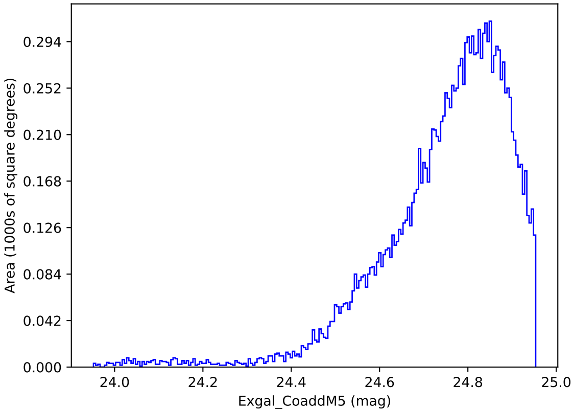
too_5_4v3.4_10yrs WFD y band: Exgal_CoaddM5
