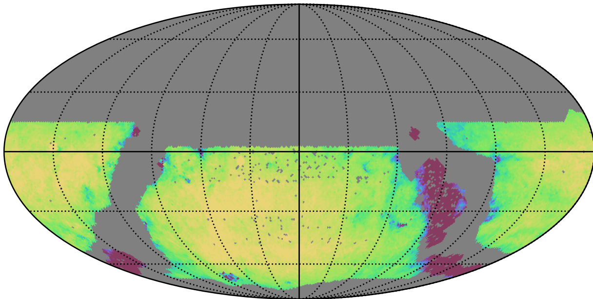
too_5_4v3.4_10yrs WFD u band: Exgal_CoaddM5
