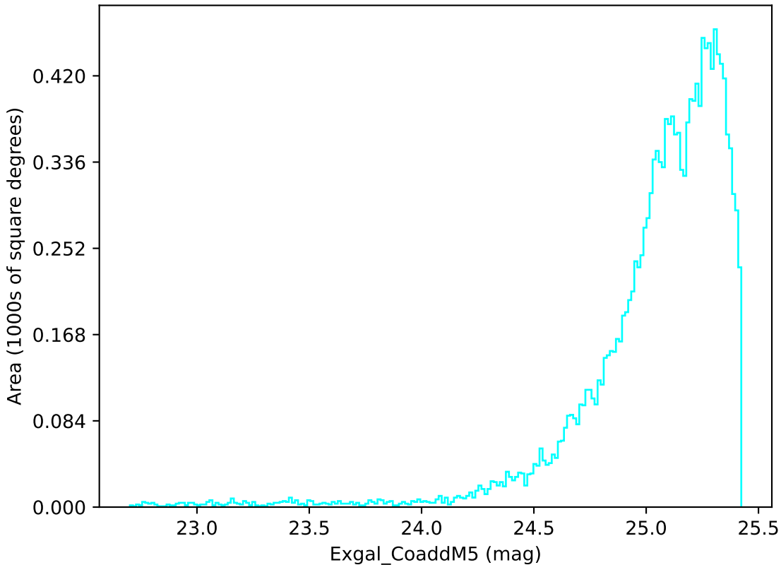
too_5_4v3.4_10yrs WFD u band: Exgal_CoaddM5
