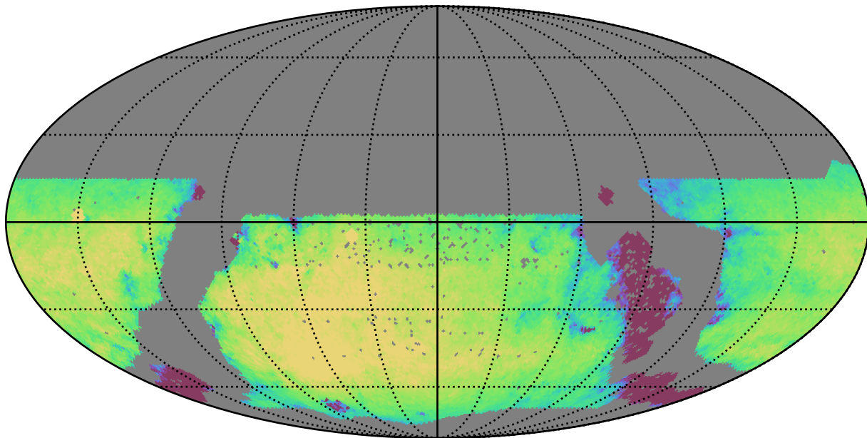
too_5_4v3.4_10yrs WFD r band: Exgal_CoaddM5
