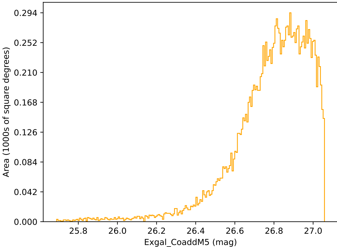
too_5_4v3.4_10yrs WFD r band: Exgal_CoaddM5
