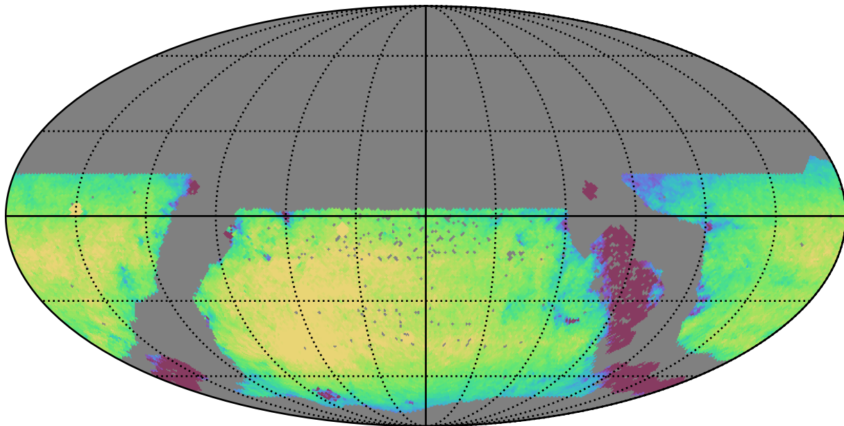
too_5_4v3.4_10yrs WFD i band: Exgal_CoaddM5
