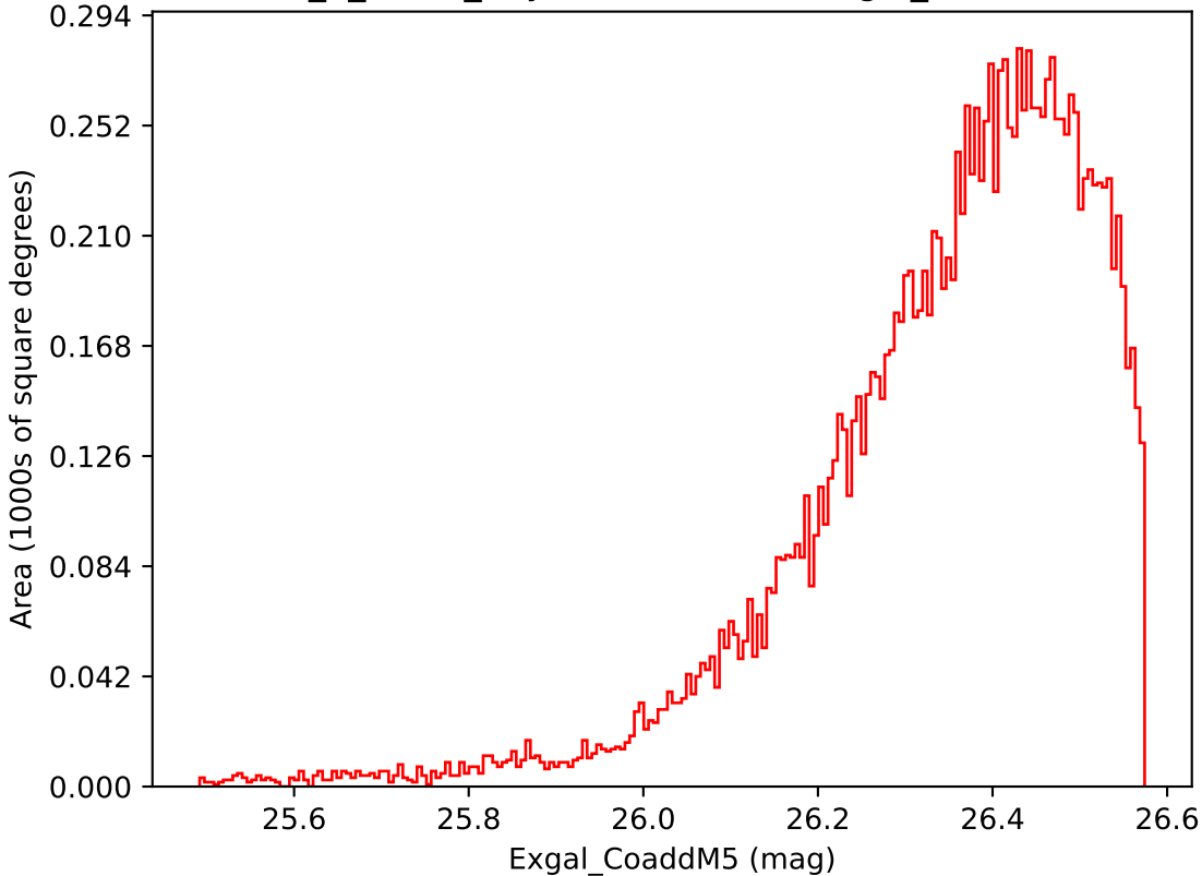
too_5_4v3.4_10yrs WFD i band: Exgal_CoaddM5
