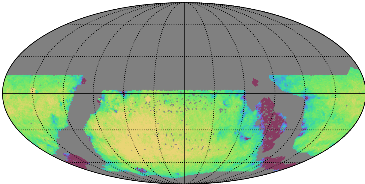
too_5_4v3.4_10yrs WFD g band: Exgal_CoaddM5
