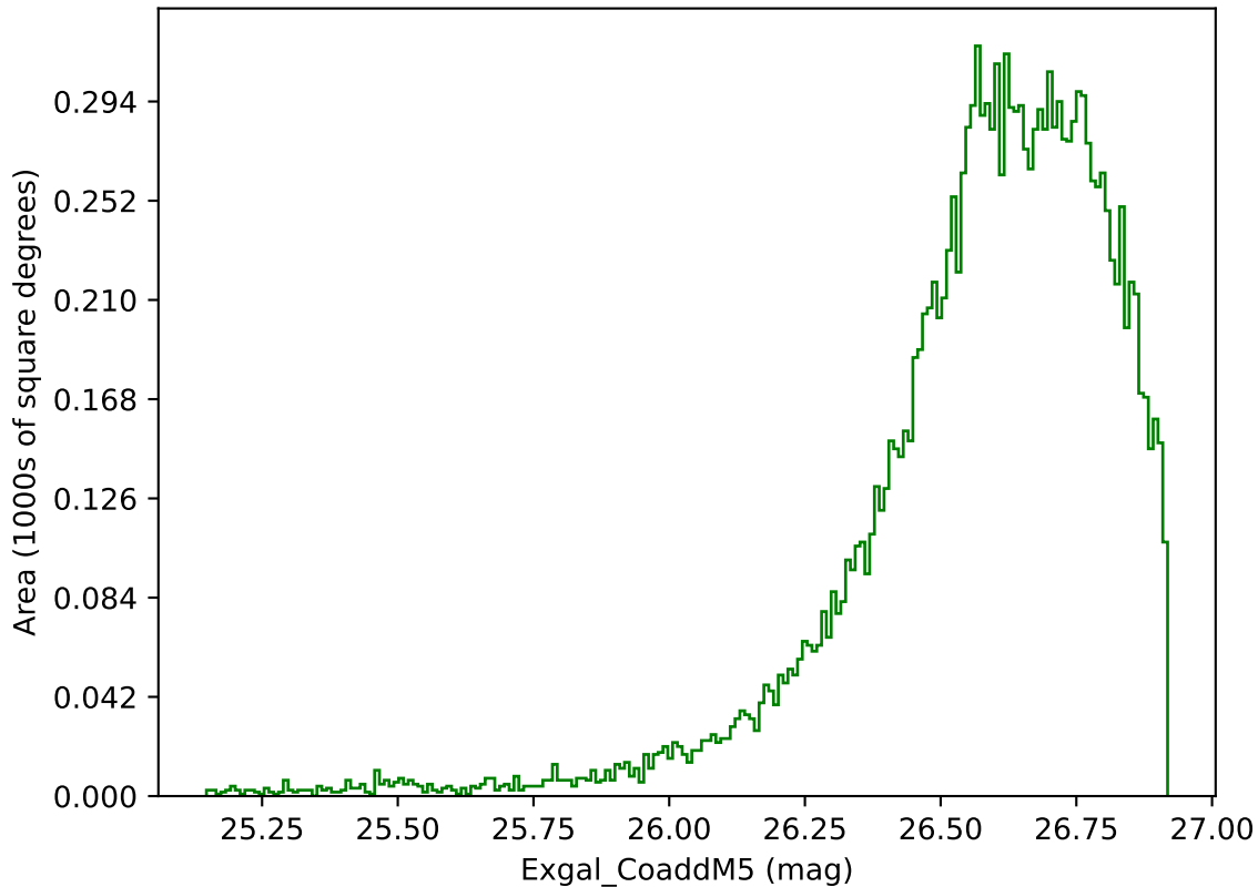
too_5_4v3.4_10yrs WFD g band: Exgal_CoaddM5
