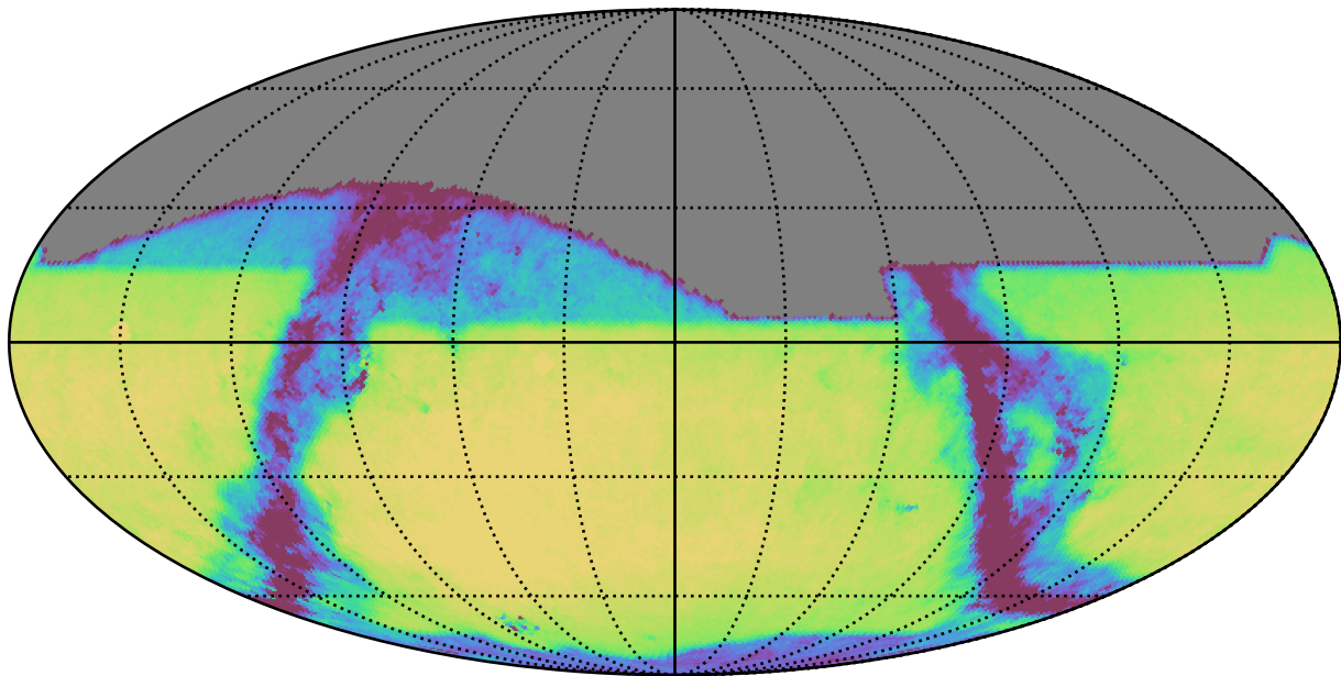
too_5_4v3.4_10yrs All sky z band: Exgal_CoaddM5
