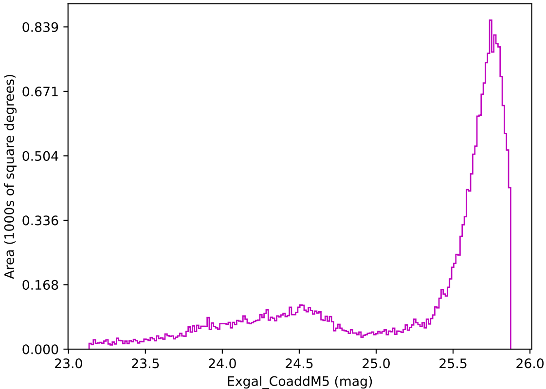
too_5_4v3.4_10yrs All sky z band: Exgal_CoaddM5
