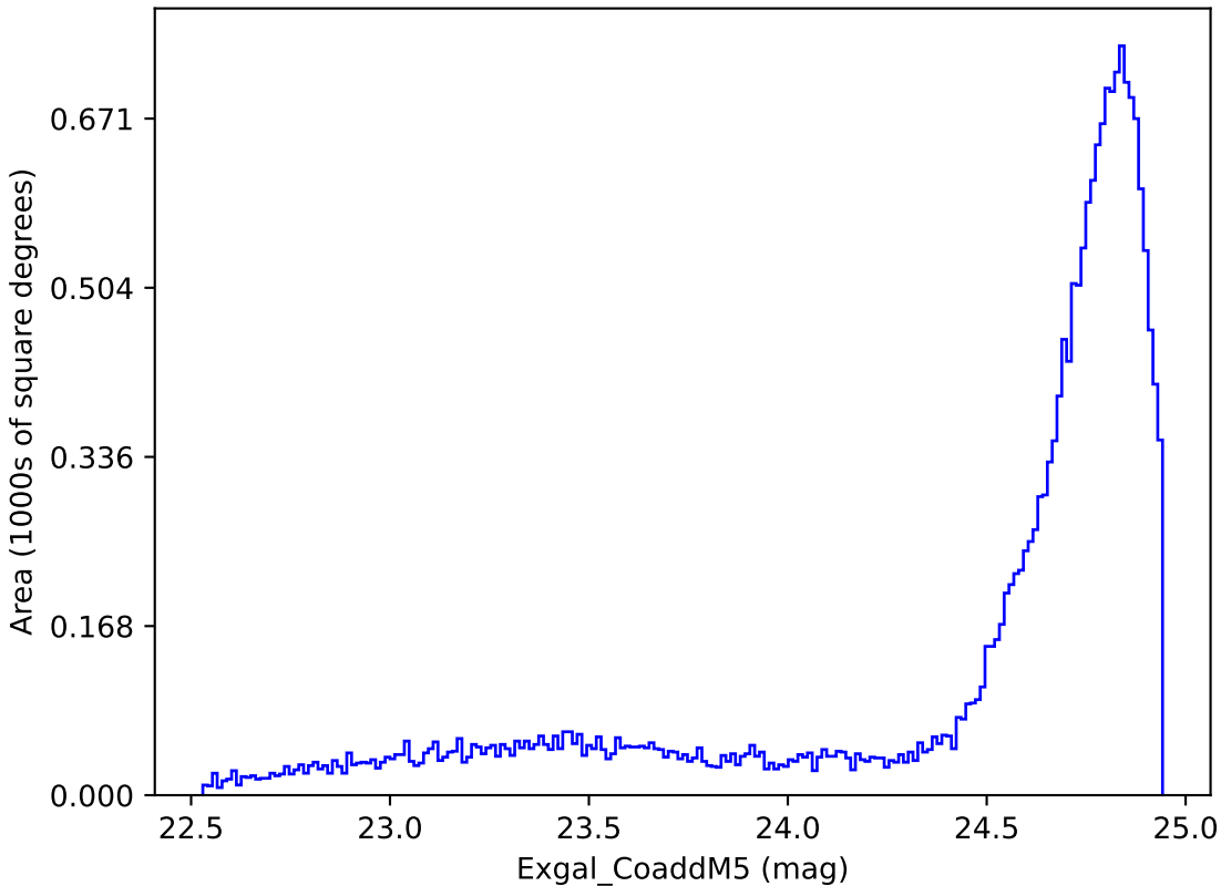
too_5_4v3.4_10yrs All sky y band: Exgal_CoaddM5
