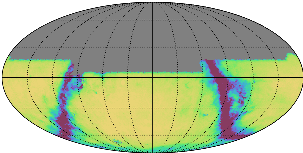
too_5_4v3.4_10yrs All sky u band: Exgal_CoaddM5
