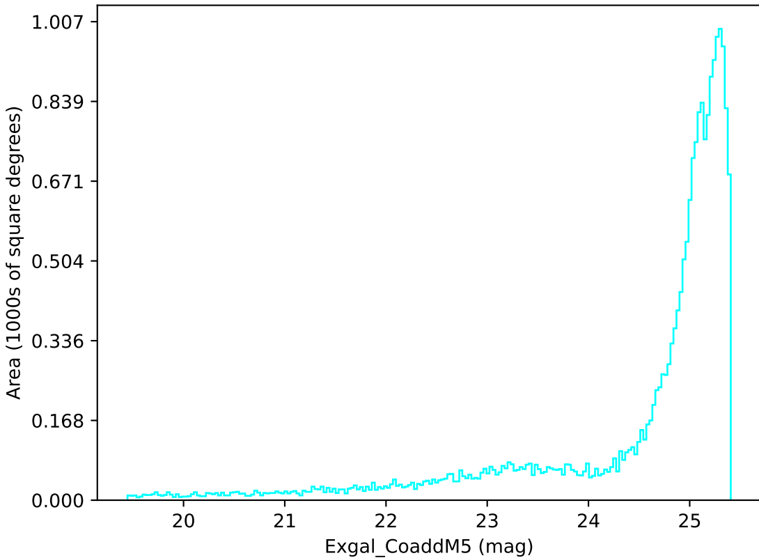
too_5_4v3.4_10yrs All sky u band: Exgal_CoaddM5
