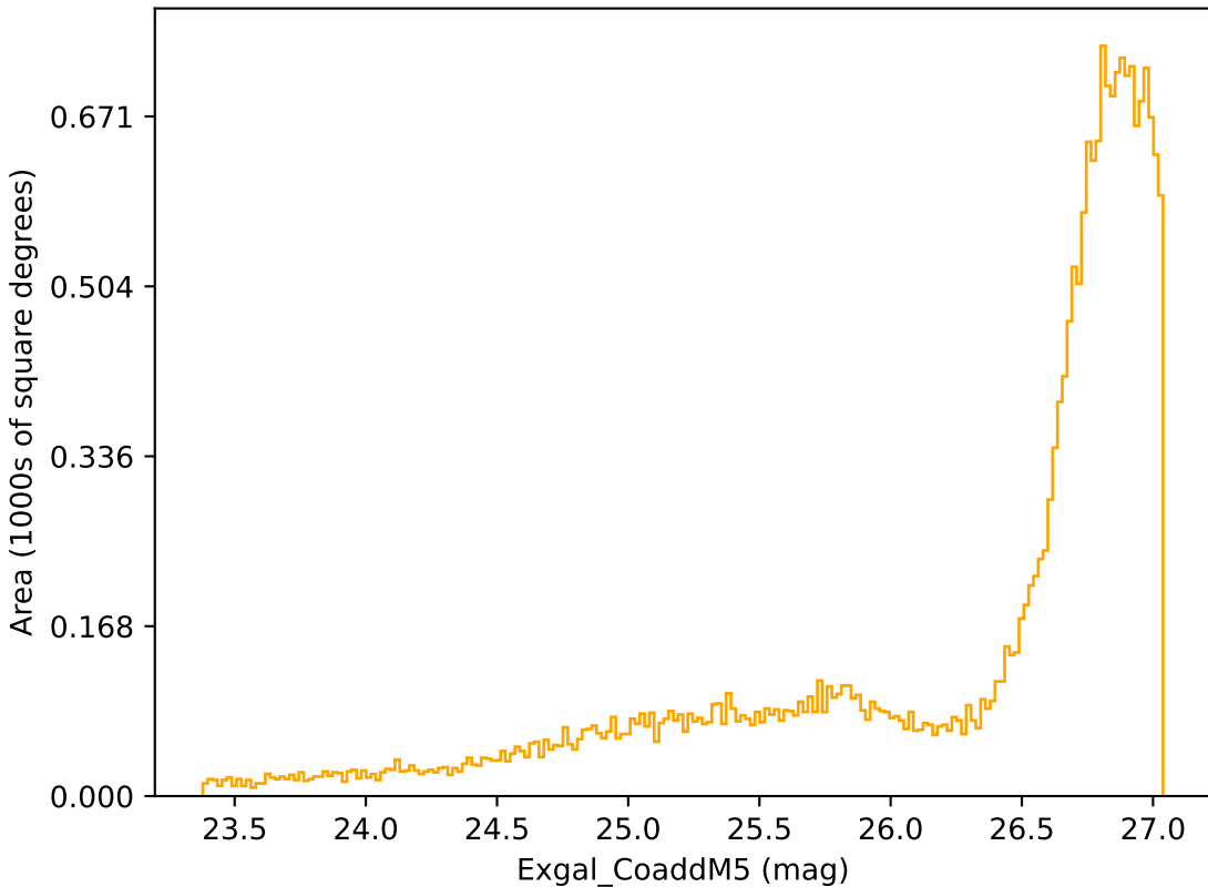
too_5_4v3.4_10yrs All sky r band: Exgal_CoaddM5
