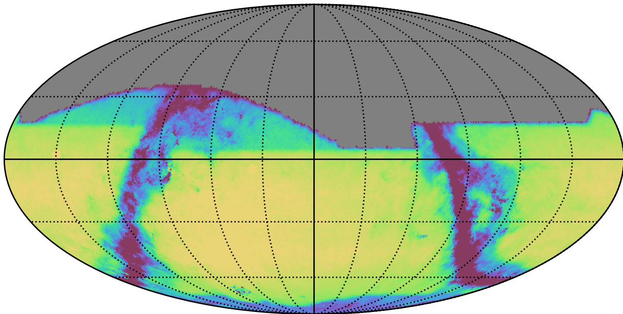
too_5_4v3.4_10yrs All sky i band: Exgal_CoaddM5
