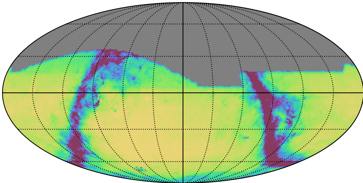
too_5_4v3.4_10yrs All sky g band: Exgal_CoaddM5
