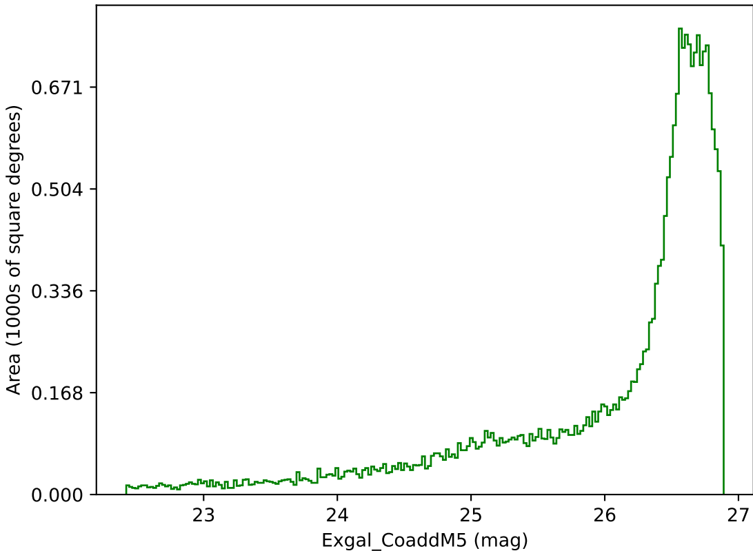
too_5_4v3.4_10yrs All sky g band: Exgal_CoaddM5
