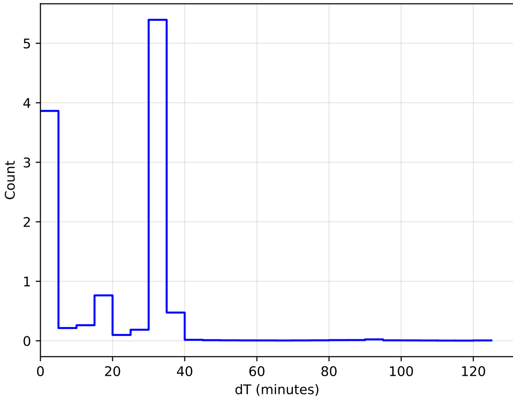
1e6 too_5_4v3.4_10yrs WFD: DeltaT Histogram
