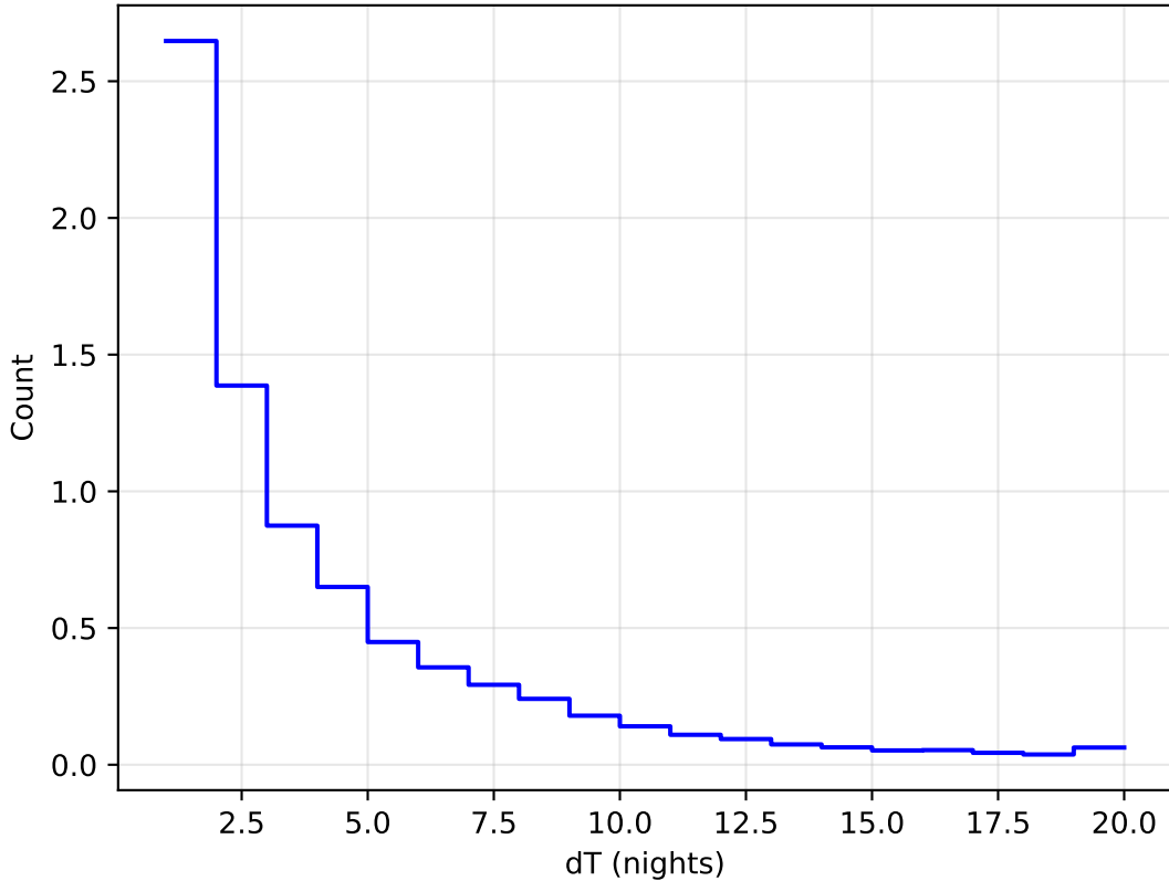
too_5_4v3.4_10yrs WFD all bands: DeltaNight Histogram 1e6
