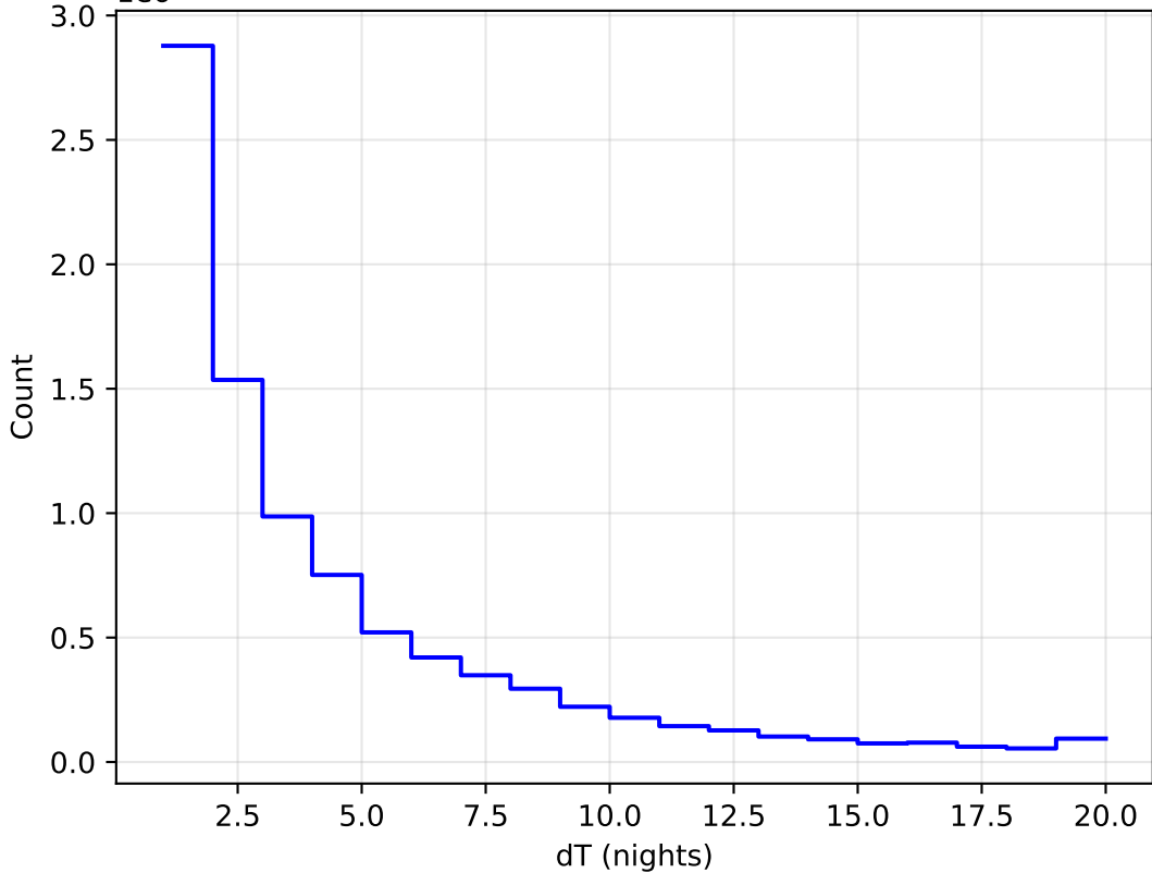
too_5_4v3.4_10yrs All sky all bands: DeltaNight Histogram 1e6
