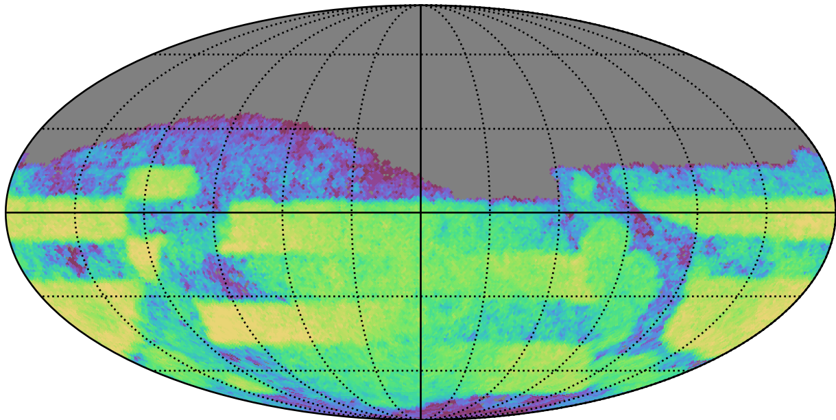
too_5_4v3.4_10yrs Yr 3-4 z band: CoaddM5
