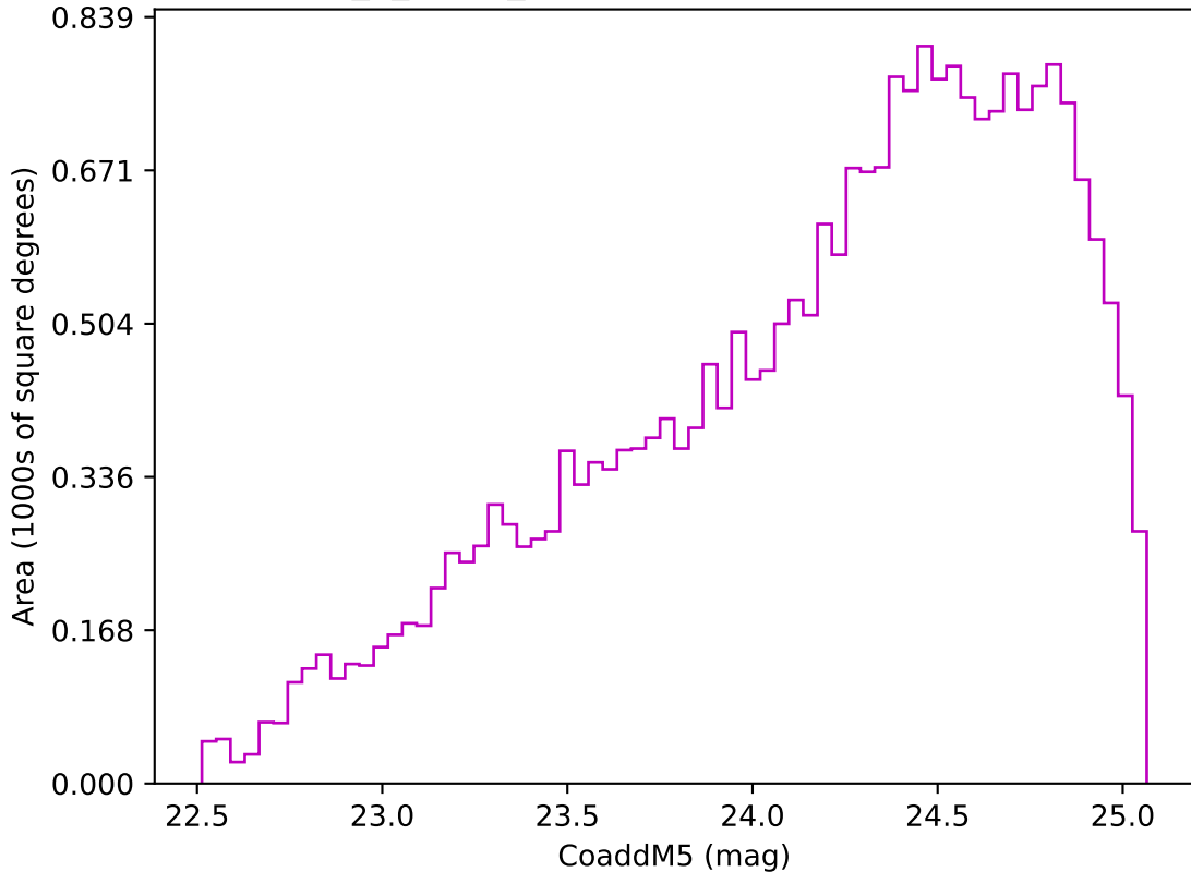
too_5_4v3.4_10yrs Yr 3-4 z band: CoaddM5
