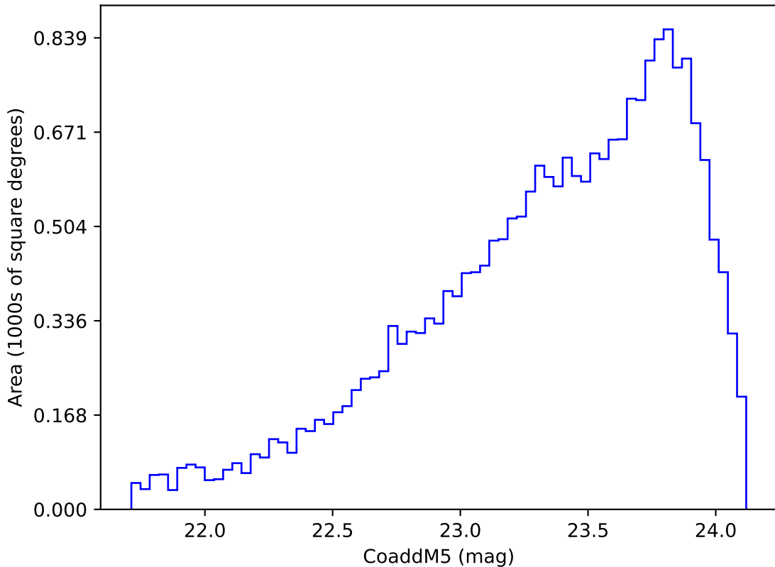
too_5_4v3.4_10yrs Yr 3-4 y band: CoaddM5
