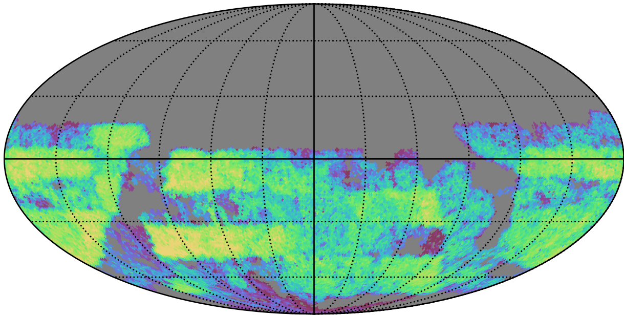
too_5_4v3.4_10yrs Yr 3-4 u band: CoaddM5
