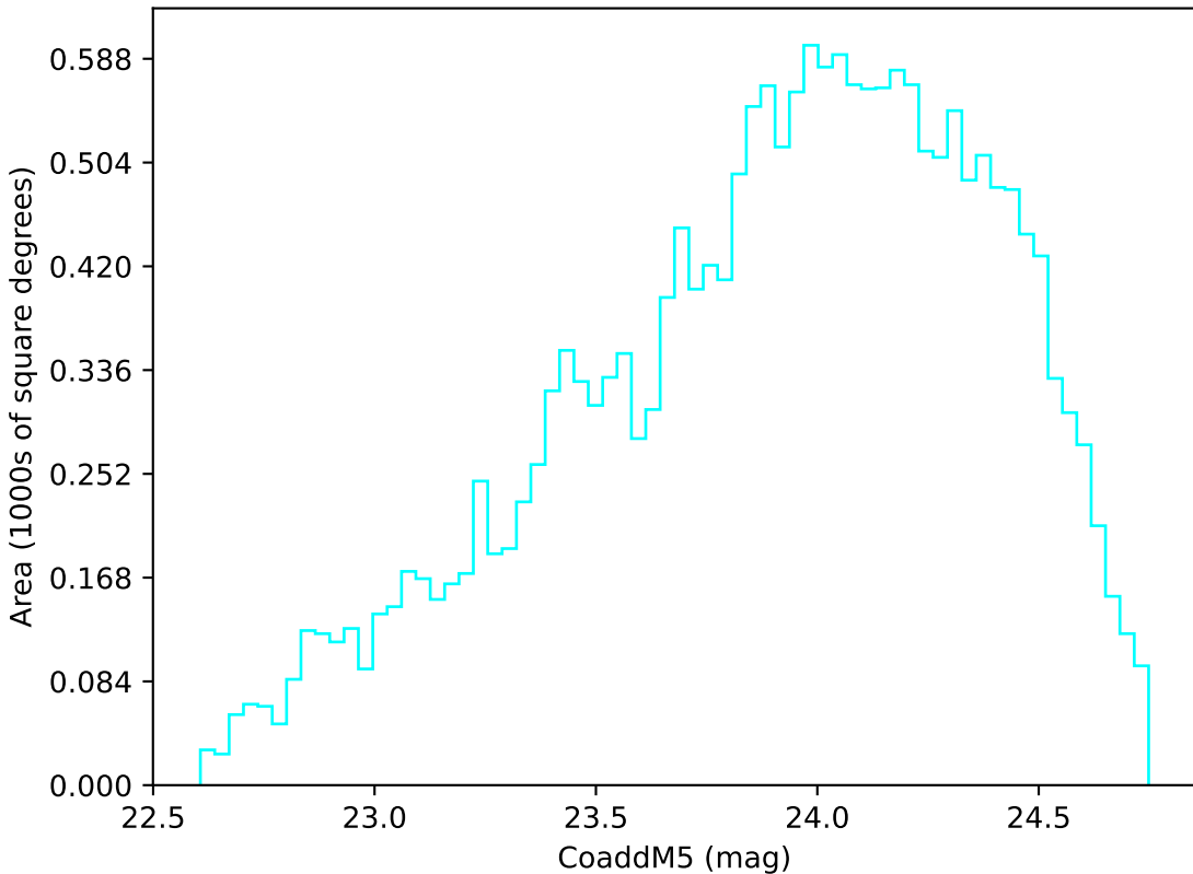
too_5_4v3.4_10yrs Yr 3-4 u band: CoaddM5
