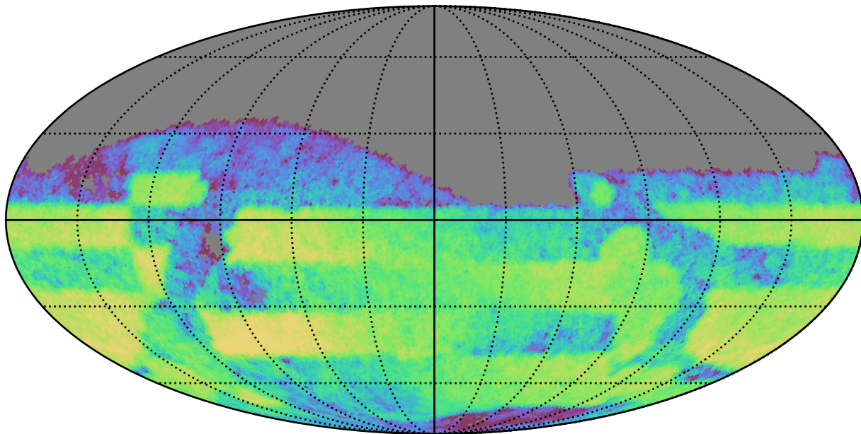
too_5_4v3.4_10yrs Yr 3-4 r band: CoaddM5
