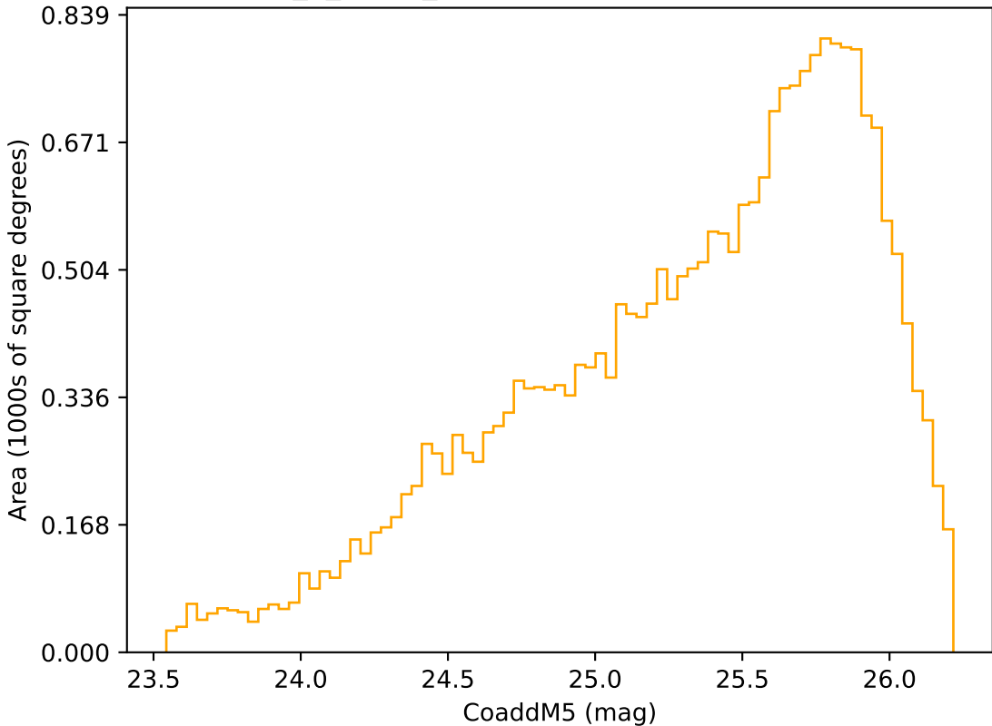
too_5_4v3.4_10yrs Yr 3-4 r band: CoaddM5
