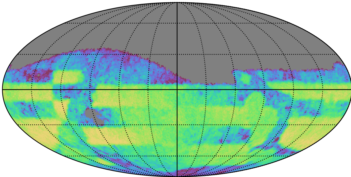
too_5_4v3.4_10yrs Yr 3-4 i band: CoaddM5
