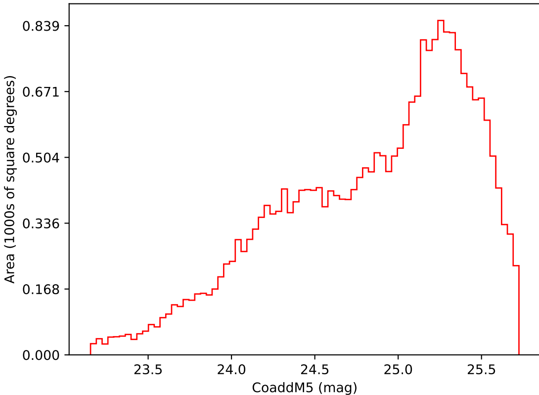
too_5_4v3.4_10yrs Yr 3-4 i band: CoaddM5
