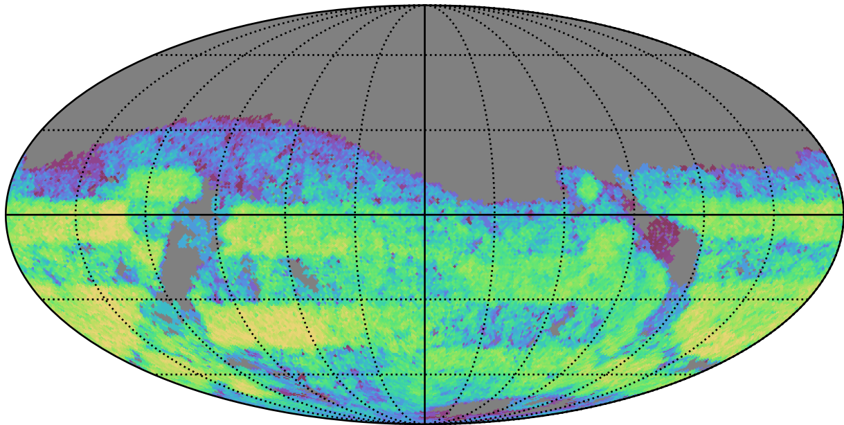
too_5_4v3.4_10yrs Yr 3-4 g band: CoaddM5
