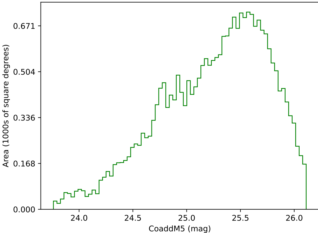
too_5_4v3.4_10yrs Yr 3-4 g band: CoaddM5
