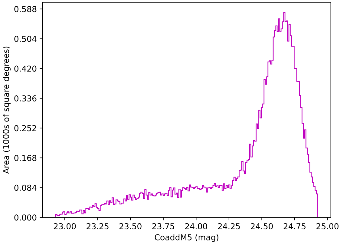
too_5_4v3.4_10yrs Yr 1 z band: CoaddM5
