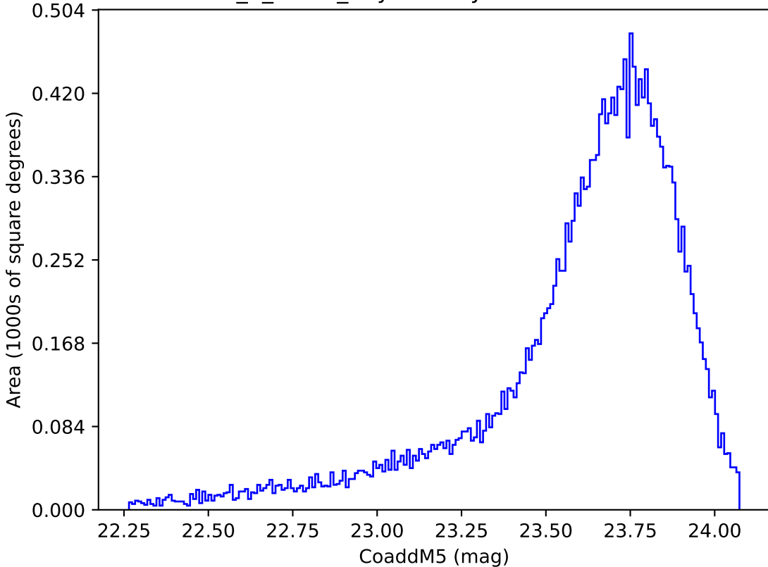
too_5_4v3.4_10yrs Yr 1 y band: CoaddM5
