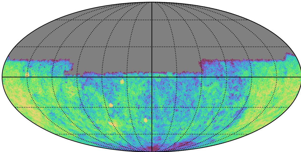
too_5_4v3.4_10yrs Yr 1 u band: CoaddM5
